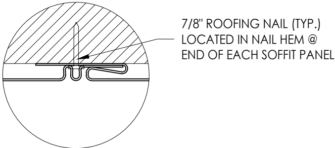
DETAIL "J"
