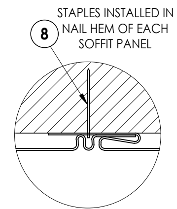
DETAIL "K"
